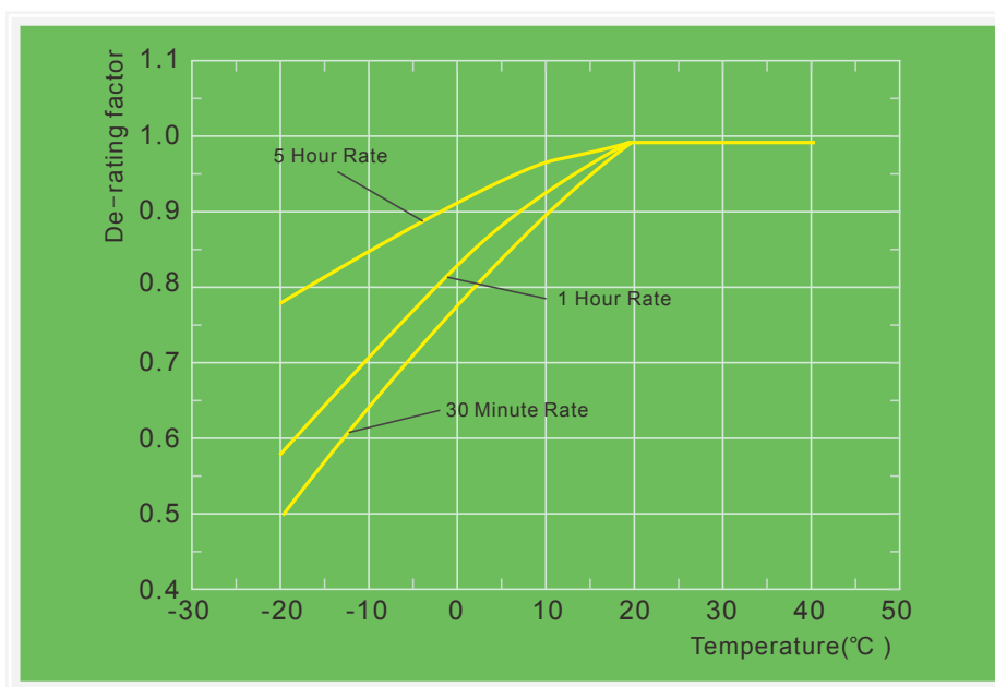
Temperature Effect Curves of SPM Series
