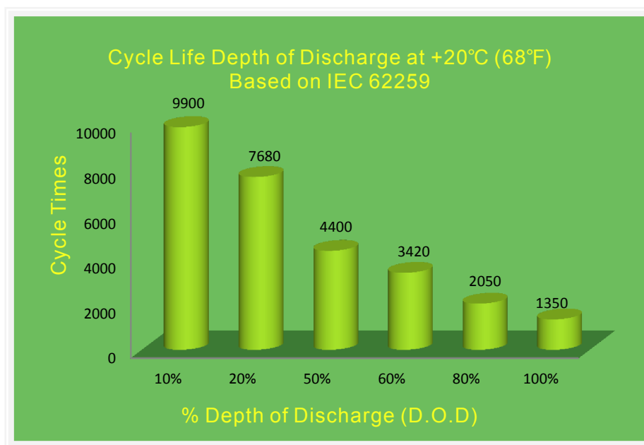
Deep of Discharge Curve of SPM Series
